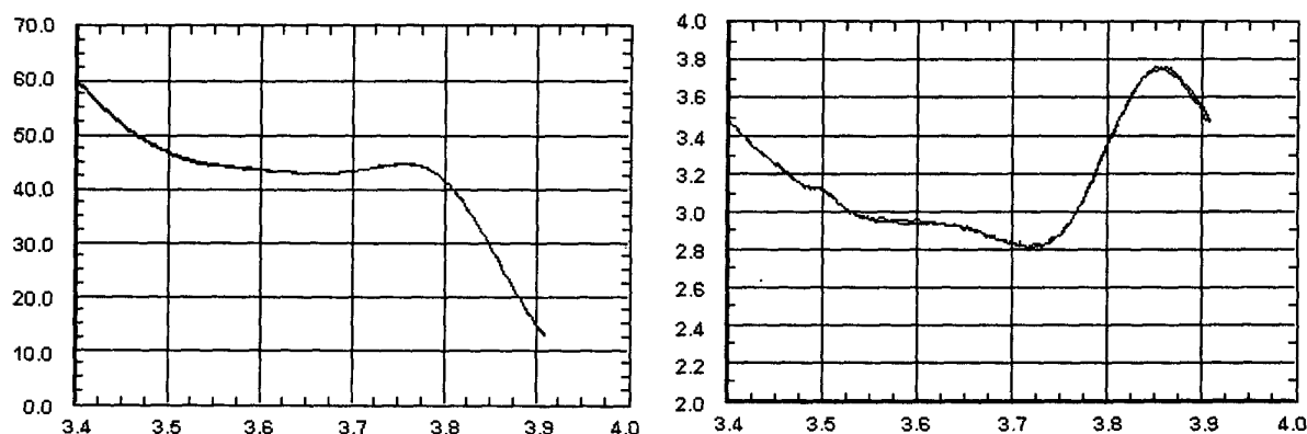
Figure 3a: Linear phase response of characterized mixer 3b: Group delay response (ns) of characterized mixer; measured as both an up-converter and as a down-converter
