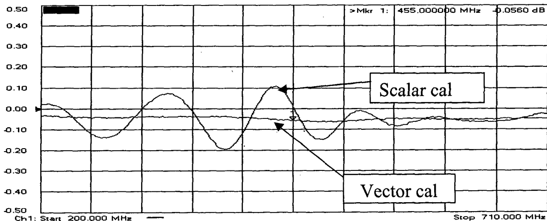
Figure 4: This shows the improvement in the mixer measurement of a mixer-plus airline, as compared with a scalar calibration technique
