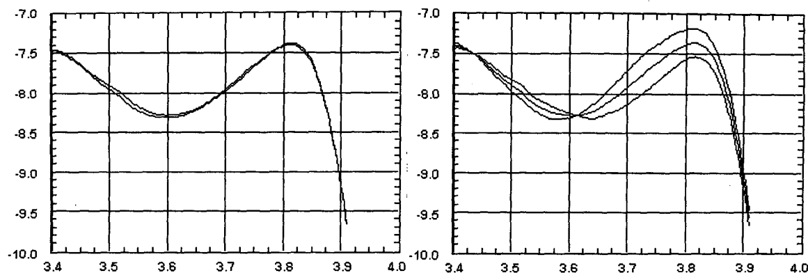
Figure 2a: Mixer conversion with the new method, measured as an up-converter and a down-converter Figure 2b: Measuring the mixer with a power meter, with a third trace showing the average of up and down conversion.
