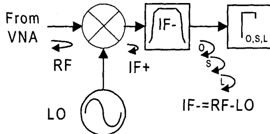
Figure 1: Mixer characterization diagram. Three measurements are made: open, short, and load response.
